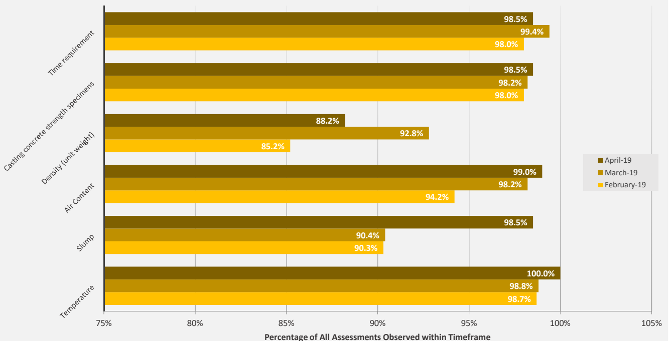
CRMCA Concrete Testing Assessment Program Field Concrete Testing Procedures Meeting Requirements in Last 3 Months
