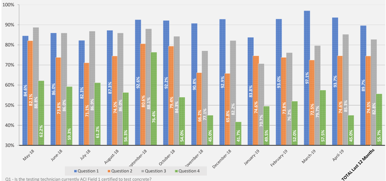
CRMCA Concrete Testing Assessment Program Percentage of Each Question Meeting Requirements in Last 12 Months
