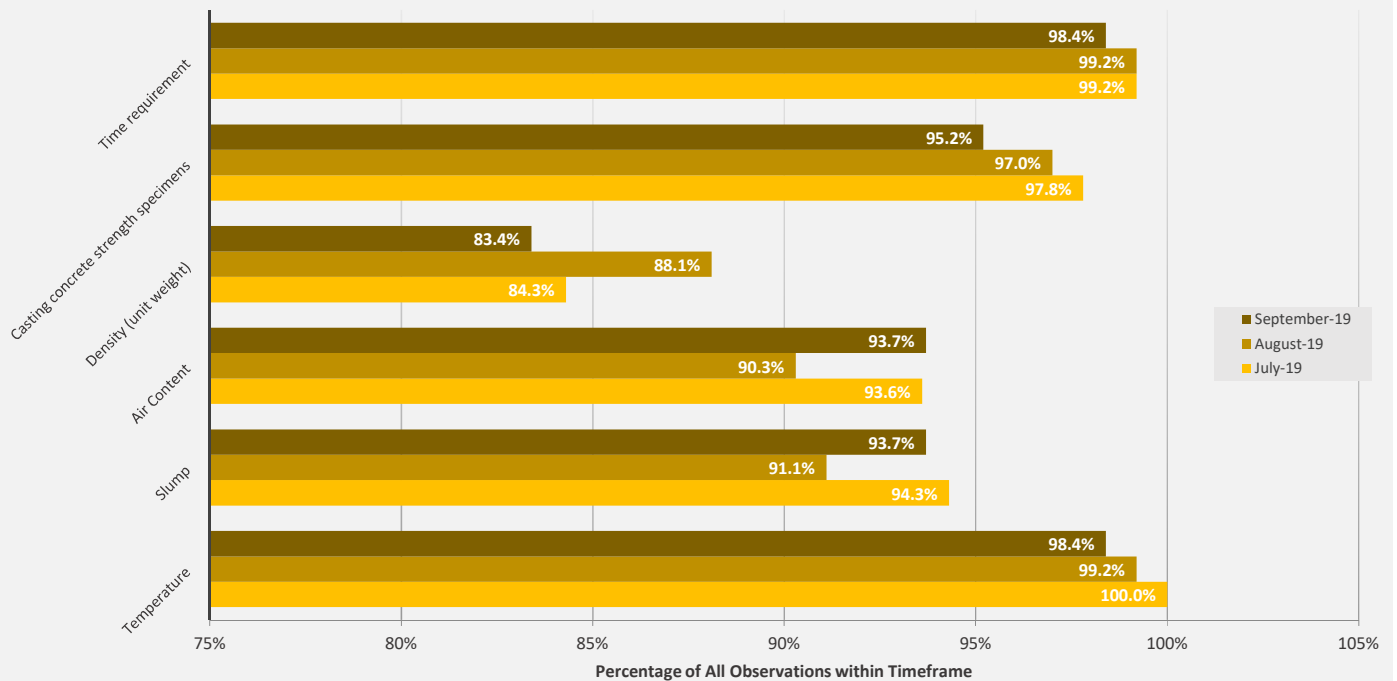
CRMCA Concrete Testing Adherence Collaboration Program Field Concrete Testing Procedures Meeting Requirements in Last 3 Months
