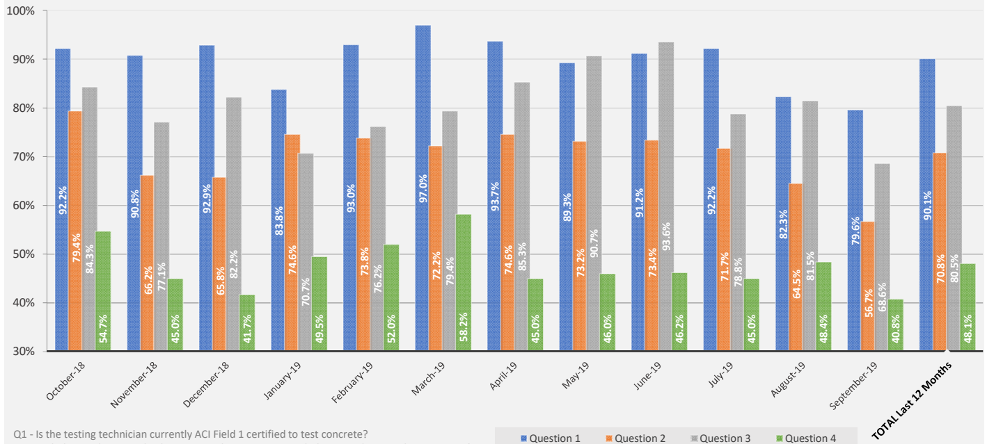
CRMCA Concrete Testing Adherence Collaboration Program Percentage of Each Question Meeting Requirements in Last 12 Months
