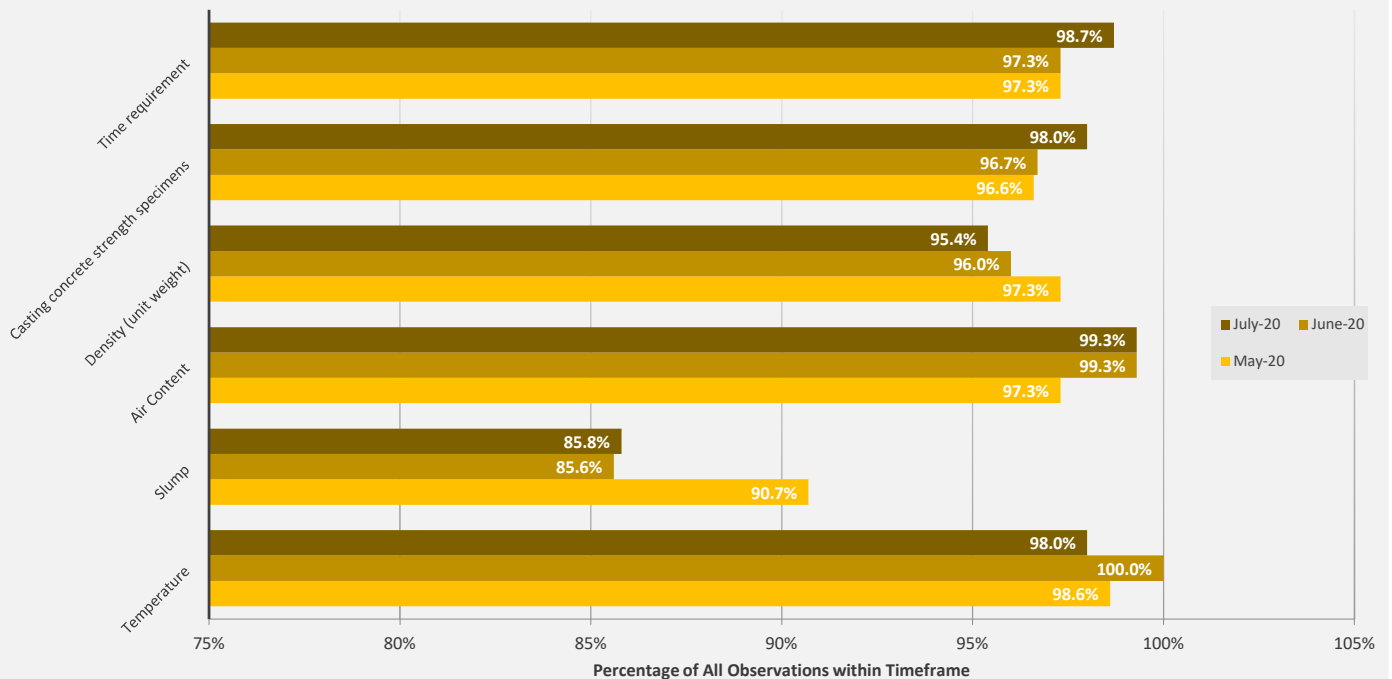
Concrete Testing Adherence Collaboration (CTAC) Program Field Concrete Testing Procedures Meeting Requirements in Last 3 Months
